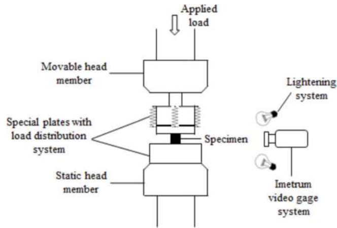
Figure 3. Quasi-static compression test setup.
