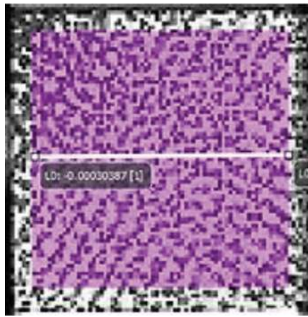
Figure 5. Inspect line L0 (middle white line) and overall area (purple square) used for DIC measurements.
