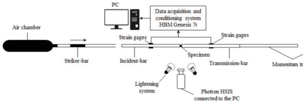
Figure 4. Schematic SHPB apparatus and HSIS set up.
