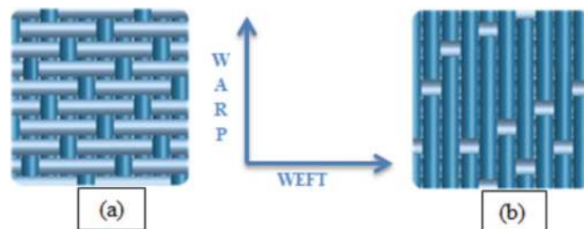
Figure 1. Harness-satin weave (a) 5HS and (b) 8HS [37].
