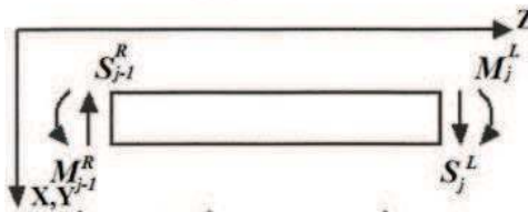
Fig. 14. The forces and moments on a field
