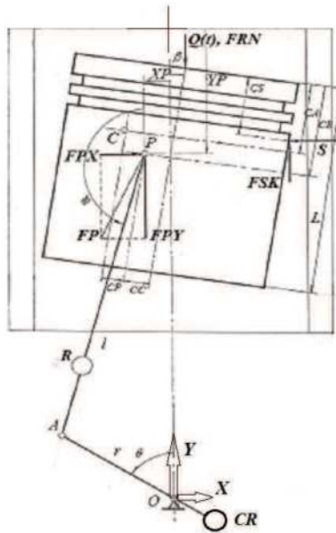
Fig. 6. Cylinder-piston-conrod-crank mechanism
