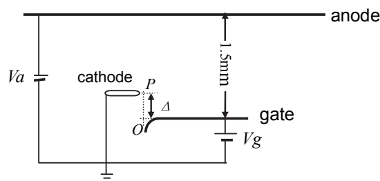
Fig. 5. Model of electric structure
