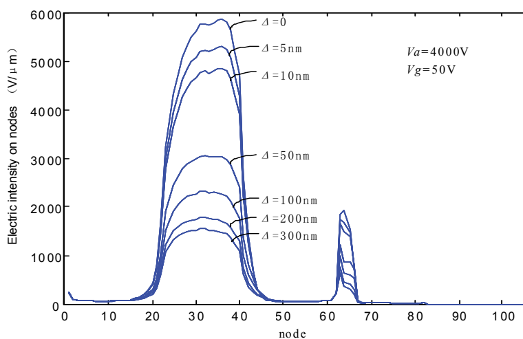
Fig. 6. Relationship of electric intensity on nodes with vertical distance between cathode and gate (the first 62 nodes on tube, the next 20 ones on gate and the last 24 ones on anode)
