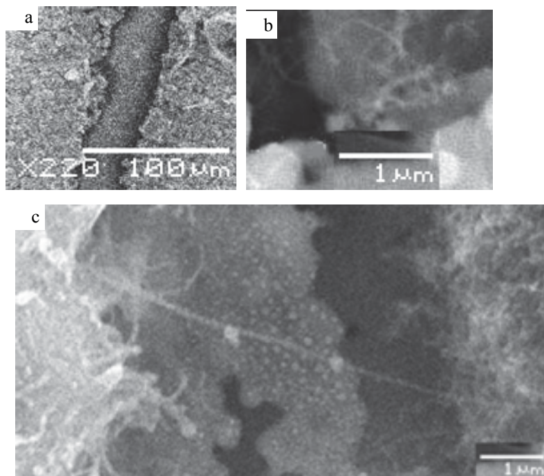
Fig. 1. (a) a trench etched with laser; (b) carbon nanotube on the edge of trench; (c) a carbon nanotube with the length of 5\mu\text{m}
