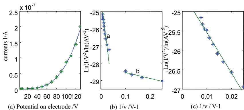
Fig. 2. (a). Emitting current vs. Voltage, (b). F-N plot (Potential ranged from 4\text{V}\sim 130\text{V} ) (c). F-N plot (Potential ranged from 40\text{V}\sim 130\text{V} )
