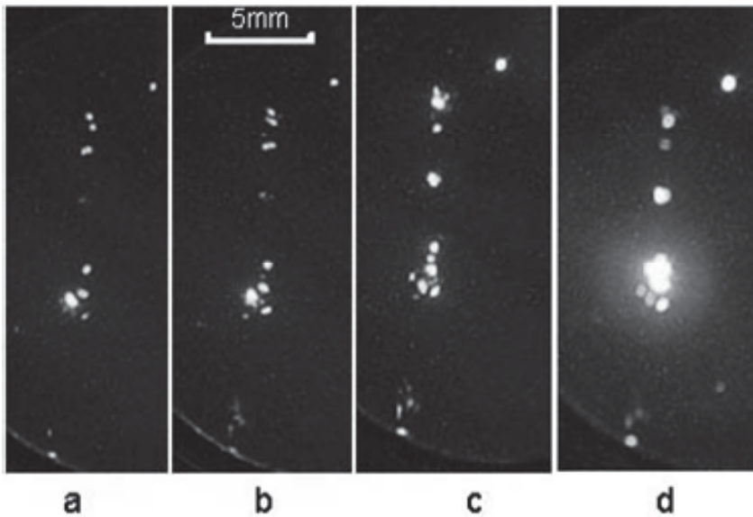
Fig. 11. a, b, c, d are light spots on the screen with different anode voltages 2.8KV, 2.9 KV, 3.0 KV, 3.2 KV respectively (voltage on gate is V_g=380\text{v} ), The cathode current I_c=1.1\mu\text{A} and the anode current I_e=0.33\mu\text{A} in Fig17c
