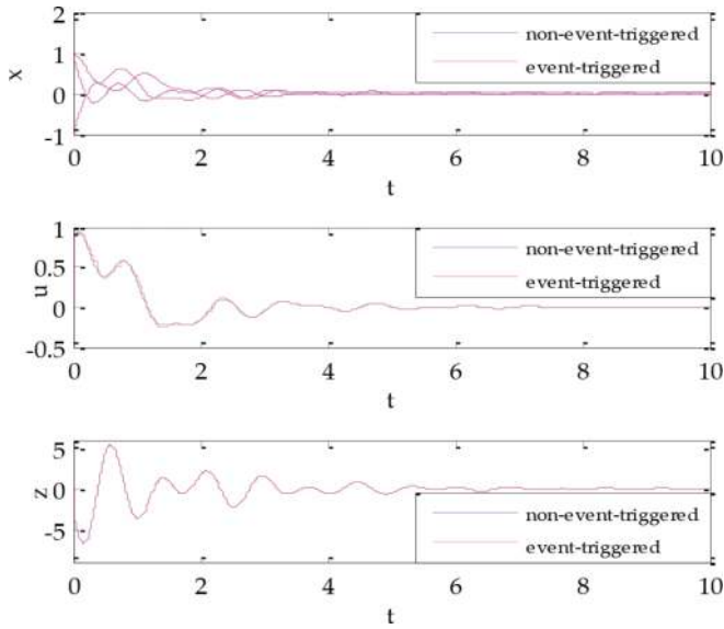
Figure 2. Responses of the second closed-loop NCS.
