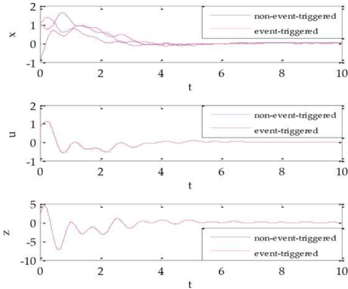
Figure 3. Responses of the third closed-loop NCS.
