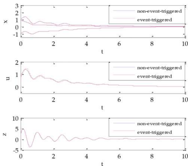
Figure 1. Responses of the first closed-loop NCS.
