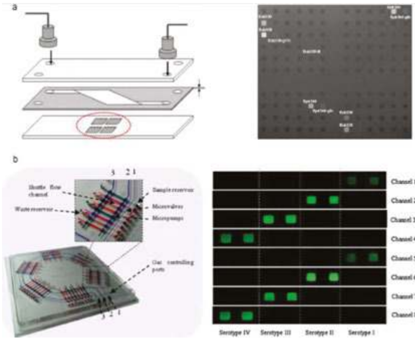
Figure 6. (a) Diagram for sample recirculation system on the hybridization chamber and hybridization image of fluorescence-labeled target nucleotide [45]. (b) Left: Photograph of the microfluidic chip containing shuttle-flow channels, microvalves and micropumps. The shuttle flow hybridization was realized by controlling the gas ports 1, 2 and 3 automatically. Right: Hybridization specificity assay using four serotypes of Dengue virus under shuttle flow conditions (frequency 2 Hz) in channels. The duration of hybridization process was 90 s and washing time was 30 s [48].
