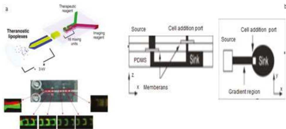
Figure 5. (a) Schematic drawing of the static micromixer-coaxial electrospay (MCE) showing its various components [37]. (b) Schematic of microfluidic gradient generator [40].
