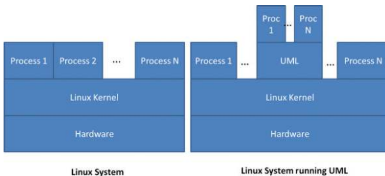
Figure 9. UML architecture (source: ICARUS).
