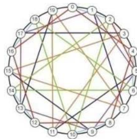
Fig. 28. Example of modified chordal ring CHR5_k(20; 4,8,4,8,2,6)
