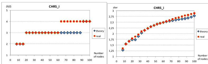
Fig. 24. Comparison of diameter and average path length of theoretical and real graphs CHR5_i
