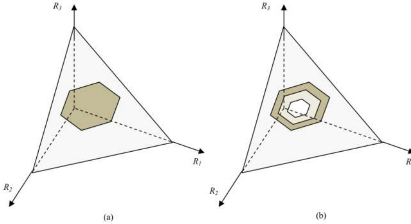
Figure 3. Feasible region.
