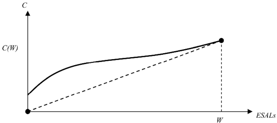
Figure 2. Cost function.
