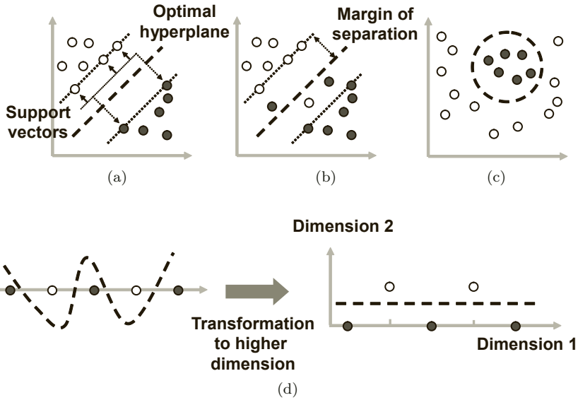
FIGURE 4.3: SVM classification problems. (a) is a linearly separable example, (b) is an non-linearly separable problem which may be solved by allowing soft margins and (c) is a completely non-linearly separable case in which linear separation may be achieved only through projection to higher dimensional space. (d) illustrates this, by showing how projecting a one dimensional space to two dimensions may make the classification linearly separable.
