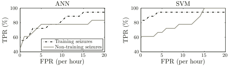
FIGURE 5.5: Average performance on Group 2 data, where the first 3 seizures are used for training and the next 3 used for testing. SVM is shown to outperform ANN when detecting seizures it has been trained on, whilst achieving similar performance to ANN when presented with unseen EEG data.
