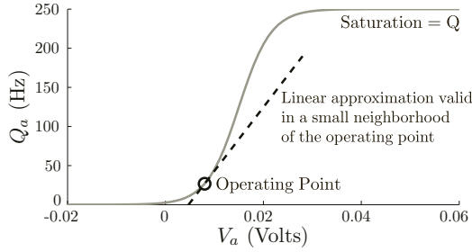
FIGURE 6.4: A typical relationship between average firing rate Q_a versus mean membrane potential V_a for ensembles of neurons of type a . Here \mathbf{Q} = 250\text{s}^{-1} , \sigma = 3.3\text{mV} and \bar{V}_{th} = 15\text{mV} . Q_a is a non-linear function that at an operating point can be approximated by a linear function as shown. This linearization is an approximation that is only valid for values close to the operating point.
