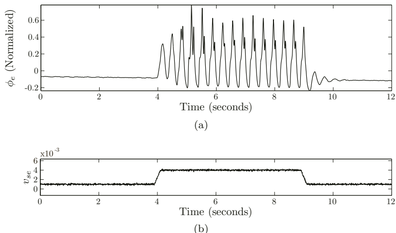
FIGURE 6.14: Sample transition in and out of system stability to replicate transitions in and out of seizure. v_{se} is varied as in (b), with additive stochastic white noise. In [22] such methods have been used to infer the importance of v_{se} on the generation of these types of seizures but its significance remains uncertain seeing as many parameters can be used to generate similar waveforms.
