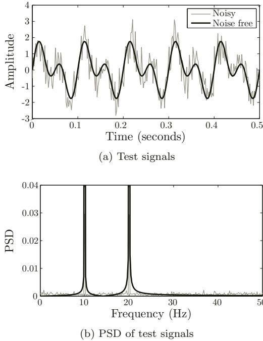
FIGURE 3.10: The power of using the FFT, as shown in (a) and (b), is its ability to reveal the frequency content in signals even in a noisy environment. The test signals are in (a) and the corresponding PSDs in (b). A sampling frequency of F_s = 512\text{Hz} is used (1 second equals N = 512 samples); thus the spectrum in (b) is defined between 0-256Hz, even though this figure shows only frequencies up to 50Hz. All PSDs are normalized to total PSD energy.
