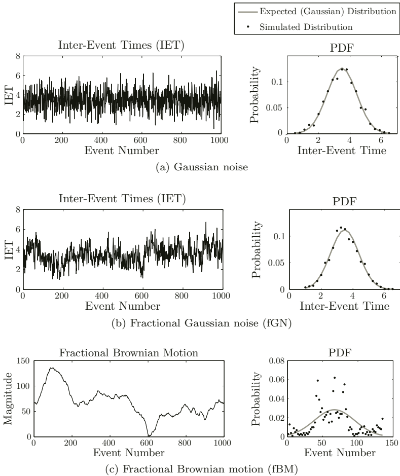
FIGURE 7.3: Simulated time series for (a) Random (Gaussian) process, (b) Fractional Gaussian Noise (fGN) with \alpha = 0.8 and (c) the consequent Fractional Brownian Motion (fBM). Upon visual inspection both the (a) and (b) look predominantly random even though some structure exists in fGN. Next to each figure is the probability density function (PDF) of the simulated time-series. (a) and (b) have similar PDFs that converge to their expected distributions quickly. The PDF of fBM, on the other hand, is more volatile and does not converge to the expected function. This is because the existence of long memory, brought about by the introduction of the parameter \alpha , makes the convergence time of the simulated time-series much longer. This is the problem when long memory exists: many data points are necessary to provide conclusive results.
