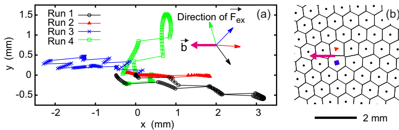
Fig. 7. Interaction of defects with large amplitude waves. (a) Simulated trajectories of isolated dislocations were placed with their initial Burgers vectors b pointing left (in -\mathbf{e}_x direction). The direction of the wave excitation force F_{ex} (and thus the wave propagation direction) is shown with the same colour as the corresponding wave trajectories. The dislocations move either in small increments due to elastic deformations of the lattice, or in large jumps due to lattice structural changes. One can see that the defect jumps occur in directions almost parallel to the Burgers vector regardless of the wave propagation direction. The crystal lattice (b) is initially characterised by a screening parameter \kappa = 0.725 . The defects are marked by ■ (7-fold defect) and ▲ (5-fold defect) and the Burgers vector by the pink arrow.
