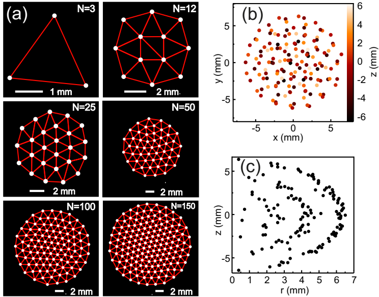
Fig. 9. Simulated Coulomb clusters in (a) 2D and (b,c) 3D. The red lines correspond to the particle bonds calculated by a Delauney triangulation, which reveals the static structure of the clusters. The numbers of particles N in the 2D clusters are shown in (a). The 3D cluster (b) has been generated using 150 particles. Its shell structure is visualised in (c) by plotting the particle positions in cylindrical coordinates ( r = \sqrt{x^2 + y^2}, z ). In (b) the colour scale corresponds to the particle's vertical position z .
