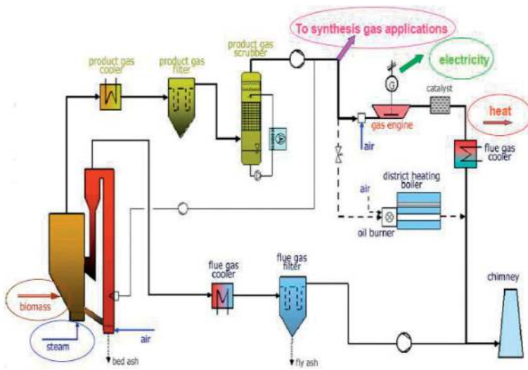
Figure 3. Process flow diagram of the gasification plant [43].
