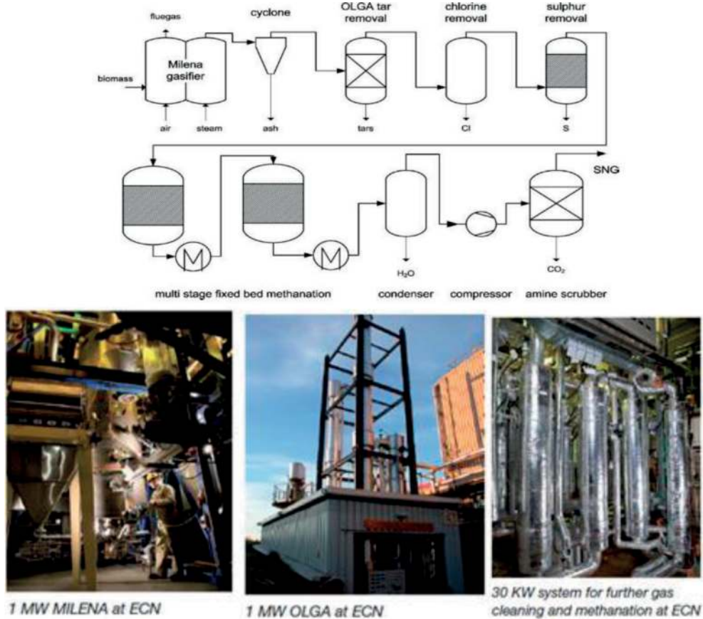
Figure 7. Process flow diagram and unit process of the ECN bio-SNG plant [47].
