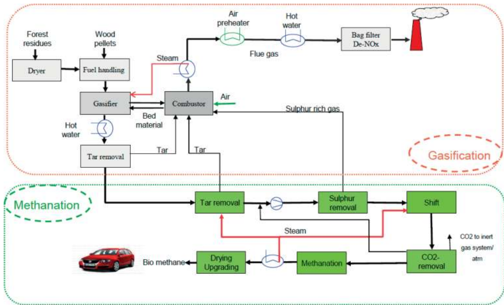
Figure 8. Process diagram of the Swedish GoBiGas plant [48].
