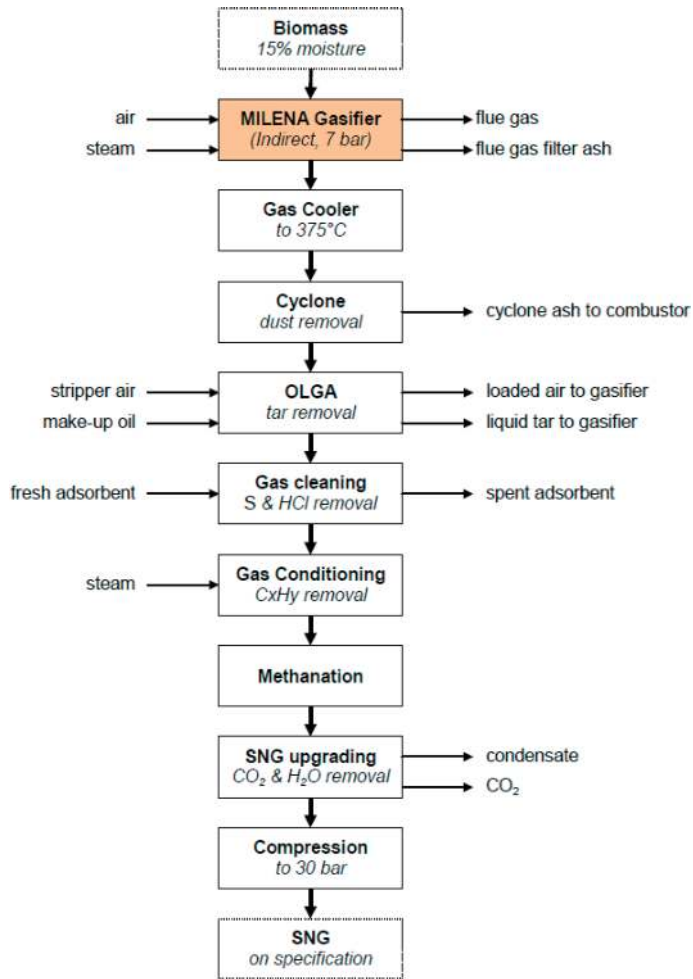
Figure 6. Process step of pilot and demo plants [45].
