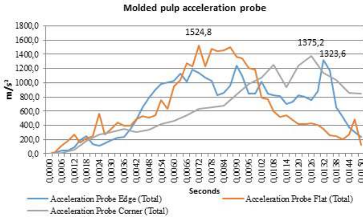
Figure 16. Molded pulp acceleration during test simulation.
