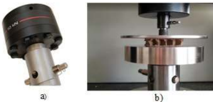
Figure 9. Instron load cell (a) and honeycomb under compression (b).
