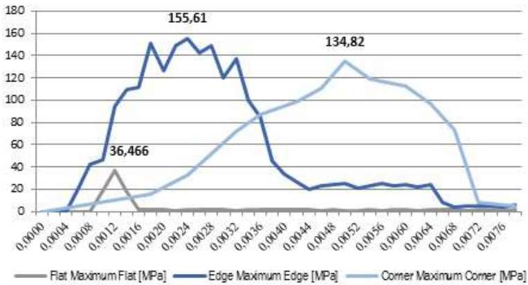
Figure 12. Equivalent stress results.
