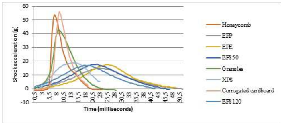
Figure 8. Highest shock for different materials.
