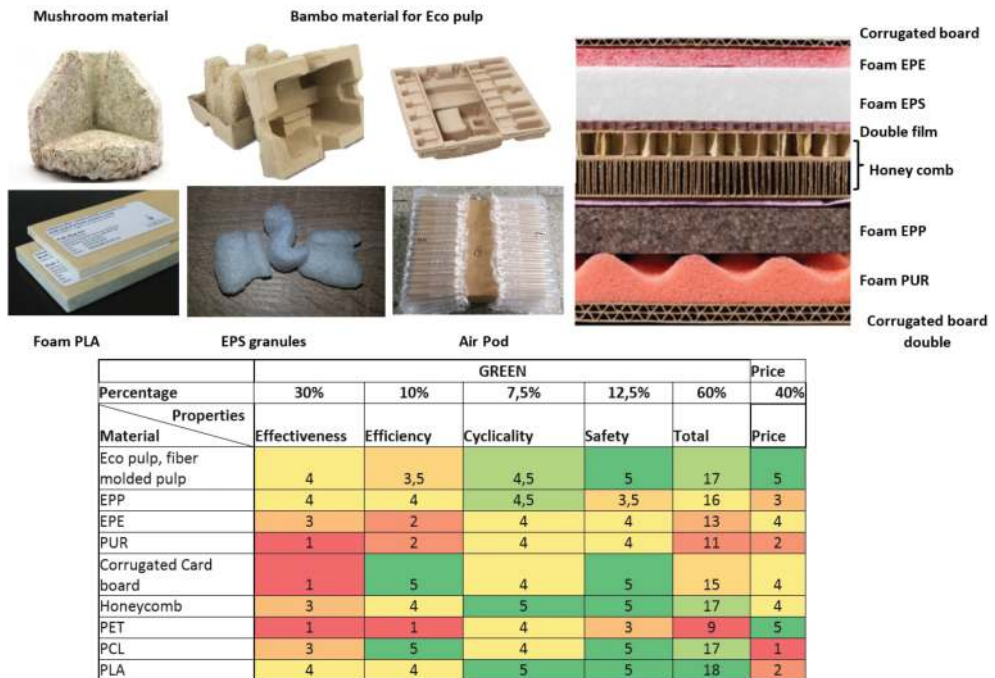
Figure 6. Materials considered for packaging.
