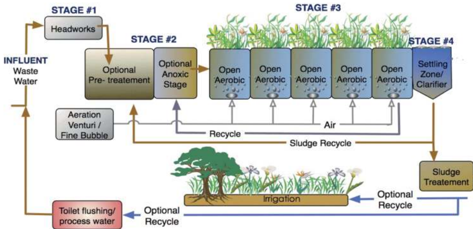
Figure 1. Ecological sewage treatment ( http://ingenious.com/sectors/the-environment/eliminating-waste-and-inefficiency/sewage-treatment-via-bionutrient-recycling/ ).
