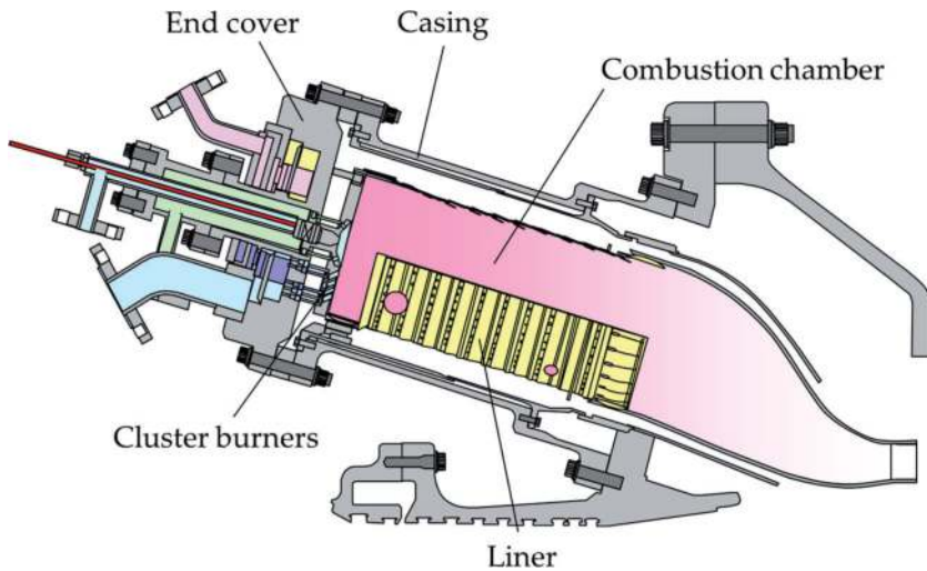
Figure 6. Cross-sectional schematic diagram of individual multi-cluster combustor.
