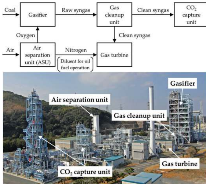
Figure 19. EAGLE pilot plant (photo courtesy of J-POWER).
