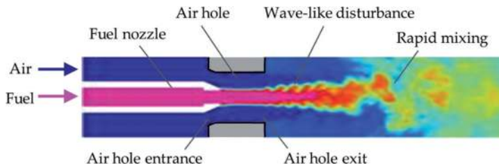
Figure 8. Mixing process of a coaxial jet.
