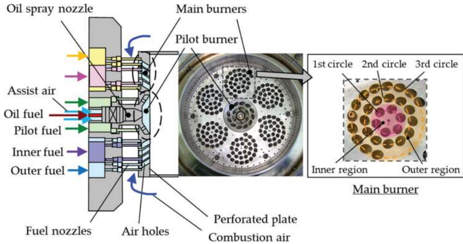
Figure 7. Detailed diagram of cluster burners.
