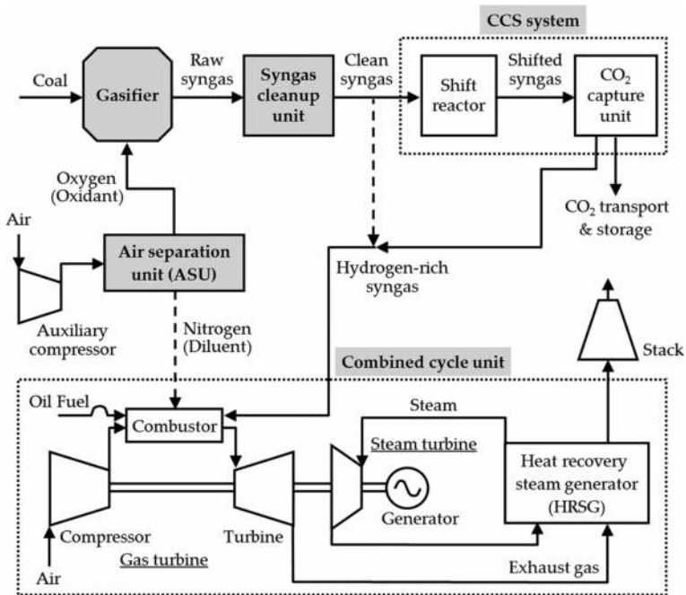
Figure 1. Schematic diagram of oxygen-blown IGCC plant with precombustion CCS system.
