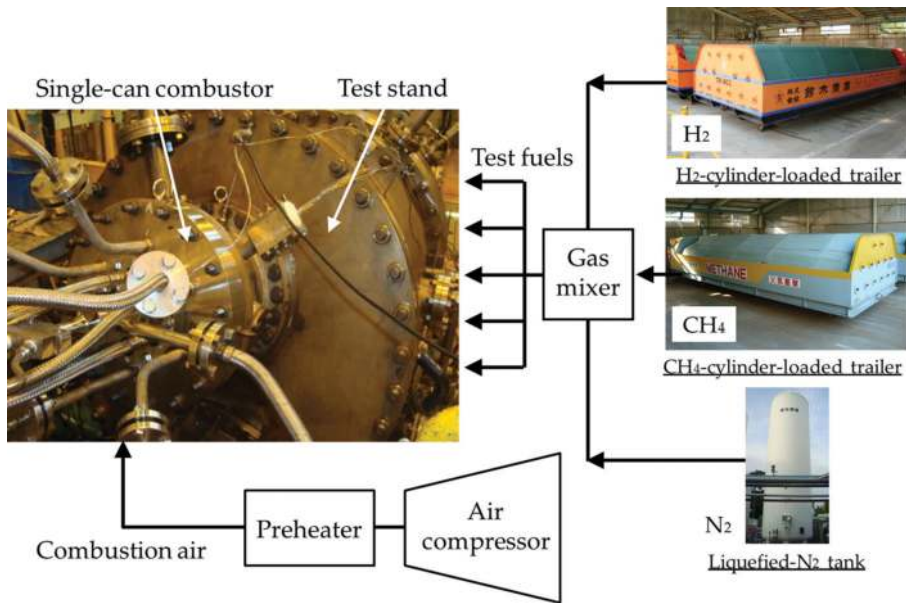
Figure 14. Single-can combustor test facility.
