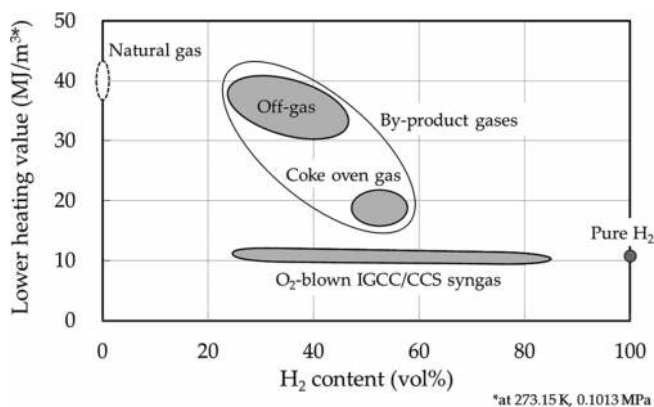
Figure 27. Suitable hydrogen-rich fuels.
