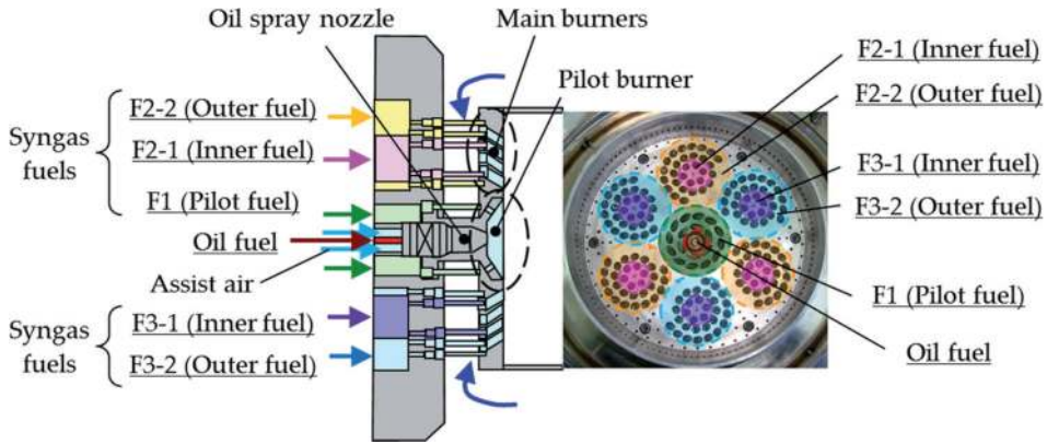
Figure 10. Fuel supplying system.
