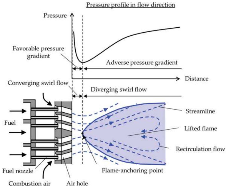
Figure 9. Operating principle of flame-lifting technology for the main burner.
