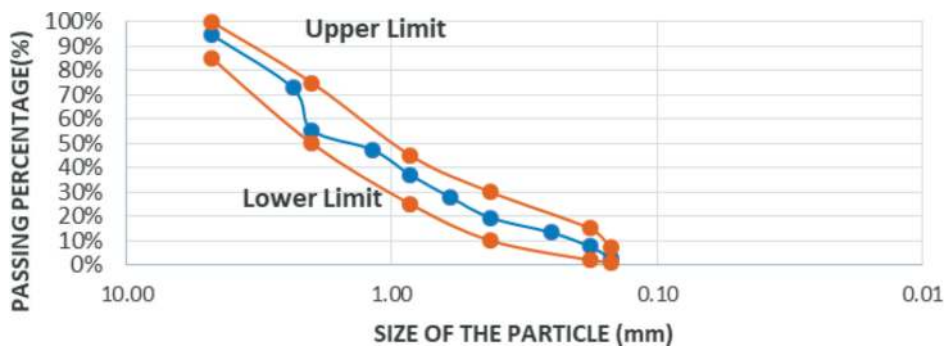
Figure 7. Granulometry of rice husk particle composition.
