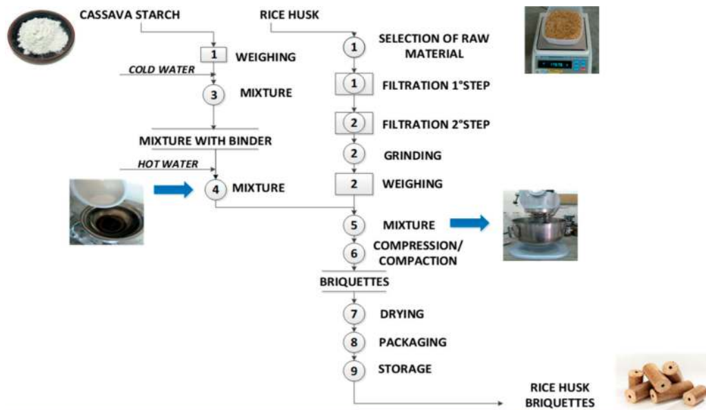
Figure 9. Rice husk briquette production process.
