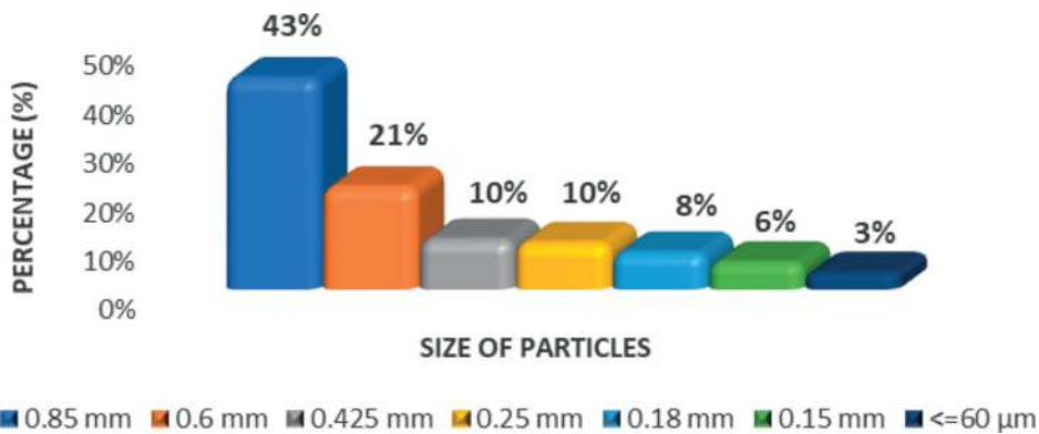
Figure 8. Granulometric distribution of rice husk particles.
