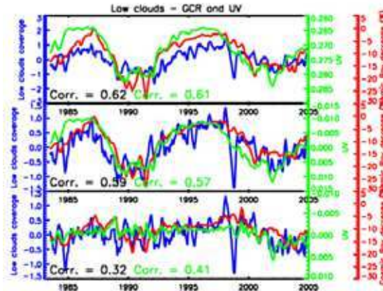
Fig. 29. Correlation between GCR (red) and UV (green) and coverage of low clouds (blue). ISCCP data for coverage of low altitude clouds after adjustment for their offset when compared with the independent data set of low cloud provided by the SSM/I microwave instrument aboard the DMSP satellites. From top: annual cycle removed, trend and internal modes removed, solar cycle removed (modified from DNSC, 2007).
