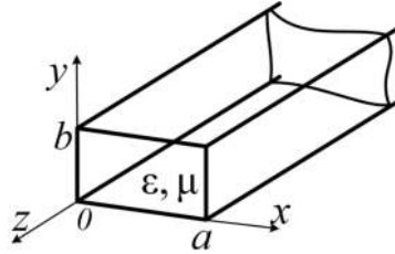
Figure 1. Rectangular waveguide (wave propagation is along z-axis).
