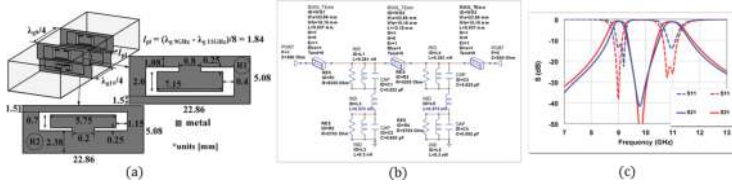
Figure 9. Second-order bandpass filter using folded metal inserts with CSRRs: (a) 3D model, (b) equivalent microwave circuit, (c) comparison of amplitude responses for the 3D EM model (blue) and equivalent circuit (red).
