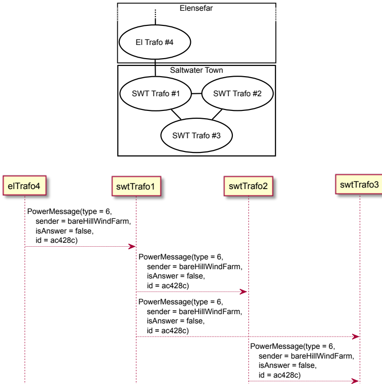
Figure 6.5: Message propagation in the ‘Saltwater Town’ part of the reference grid
