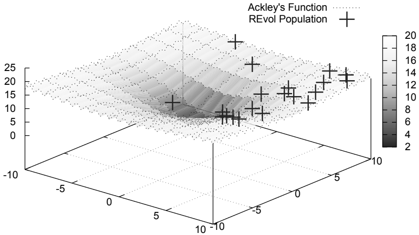
Figure 5.4: Plot of the initial population in Ackley's Function
