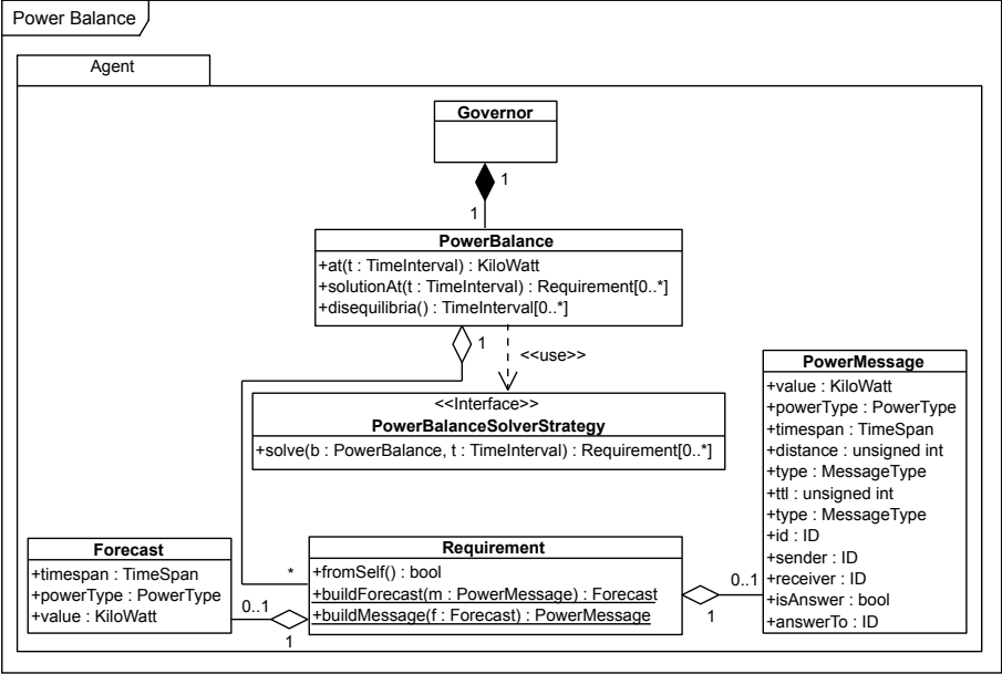
Figure 7.1: The Universal Smart Grid Agent's internal power balance
