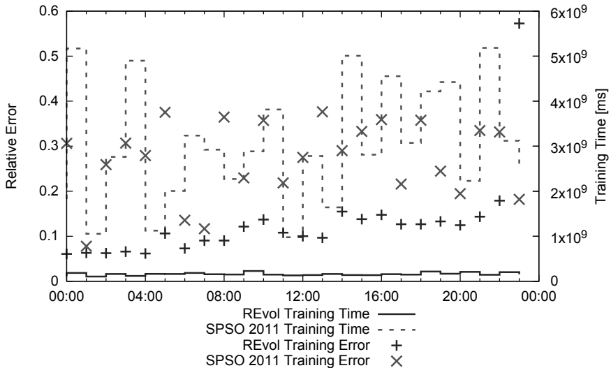
Figure 5.7: Training algorithm performance
