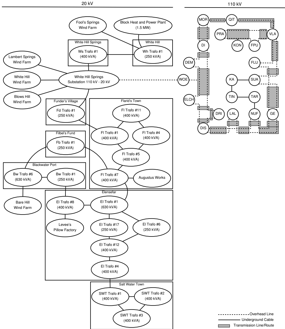
Figure 3.2: Logic view on the modeled reference power grid
