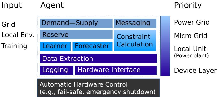
Figure 4.1: Modules of the Universal Smart Grid Agent
