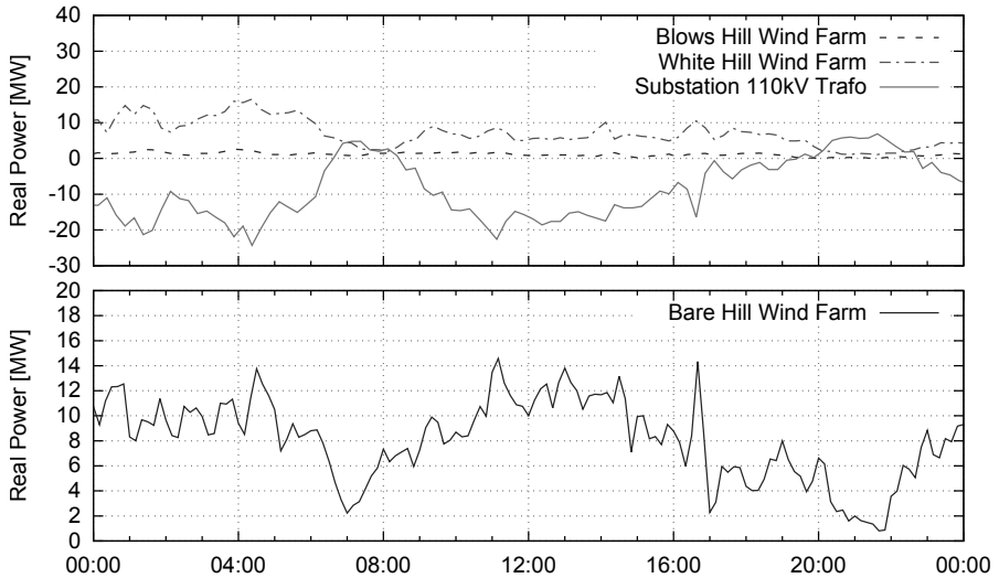
Figure 3.3: Active power at wind farms and the connecting substation during a day in February in the reference grid
