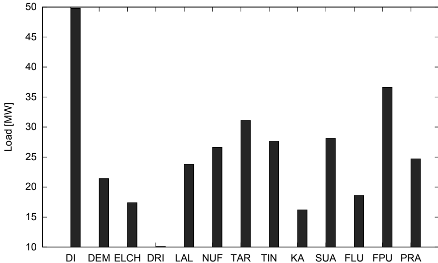
Figure 3.4: Peak load of the 110kV nodes in the reference grid
