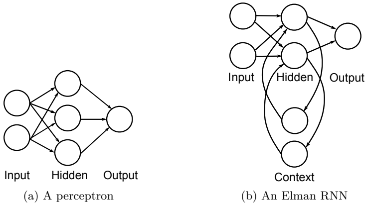
Figure 2.10: Two types of Artificial Neural Networks
