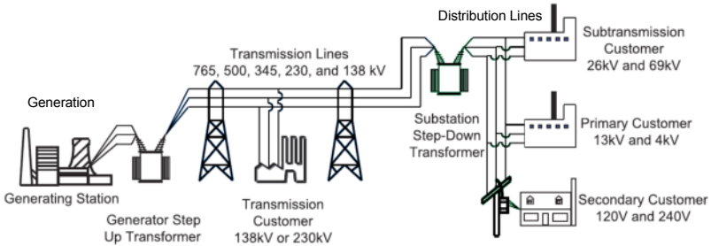
Figure 2.1: The traditional view of the power grid as one-way flow of power from generators to consumers
