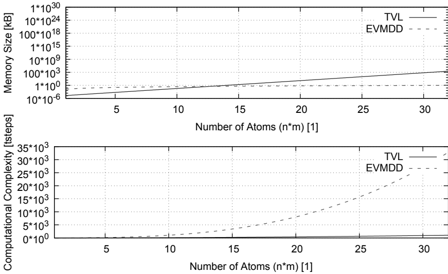
Figure 7.4: Memory size and computational complexity of XBOOLE-based and Edge-Valued Multi-valued Decision Diagram-based demand-supply solvers
