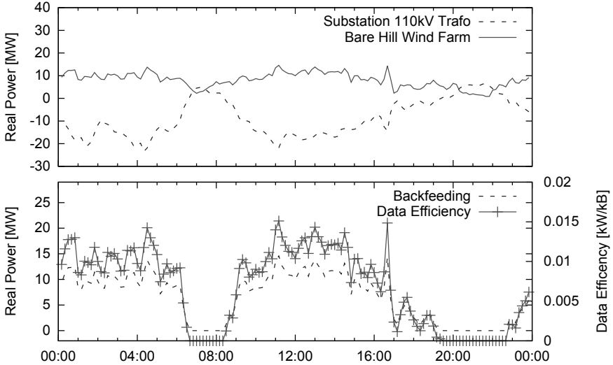
Figure 7.6: ‘White Hill Springs Substation’ backfeeding, ‘Bare Hill Wind Farm’ active power production, and data efficiency of grid-local consumption
