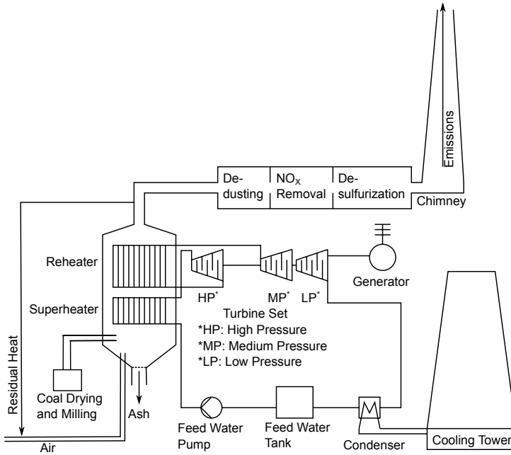
Figure 2.3: Schematic view of a coal power plant
