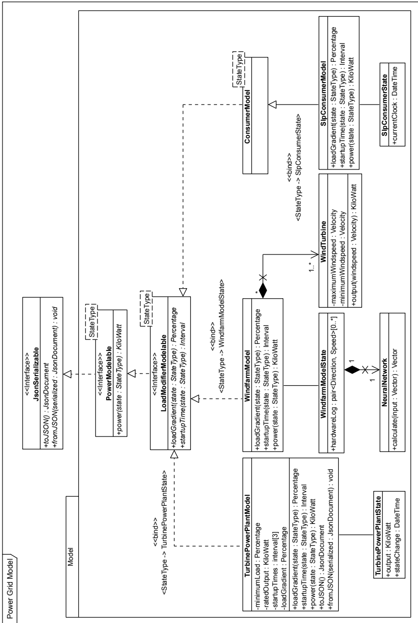
Figure 3.1: Excerpt from the simulator architecture for models and associated states
