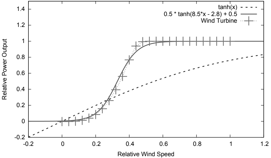
Figure 5.8: The Artificial Neural Network’s activation function and the power curve of a wind turbine
