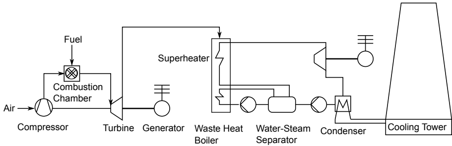
Figure 2.4: Schematic view of a combined gas and steam power plant
