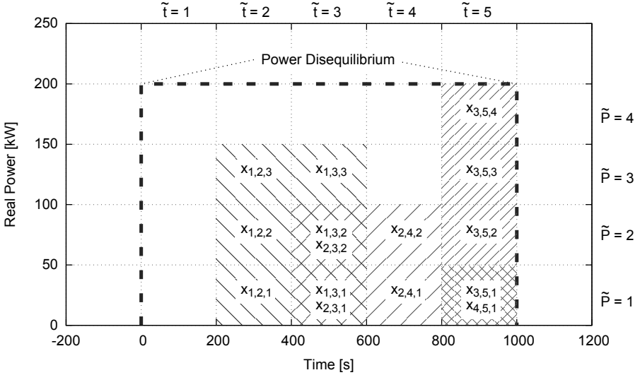
Figure 7.2: An example of a power balance state after the discretization
