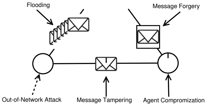
Figure 6.6: Possible attack vectors
