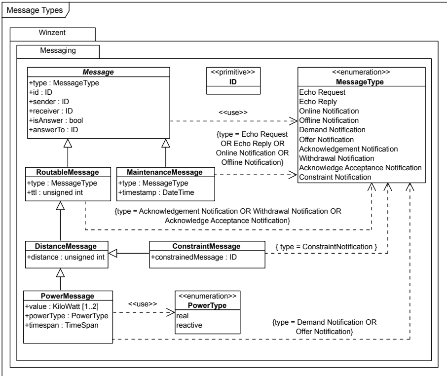
Figure 6.3: Types of protocol messages along with the class they belong to
