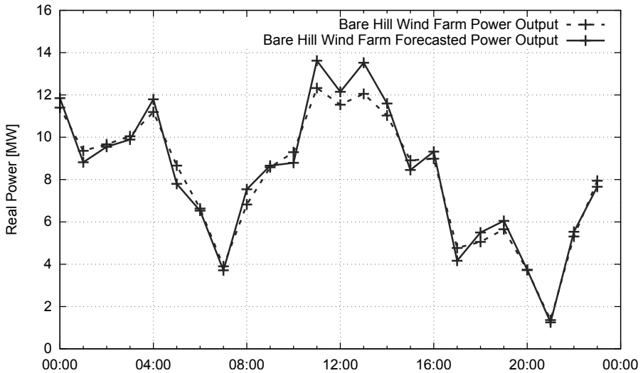
Figure 5.10: Result of node-local forecasting at ‘Bare Hill Wind Farm’
