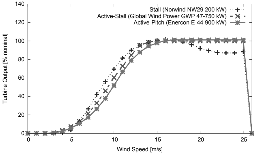
Figure 2.5: Power curves of wind turbines with different control technologies
