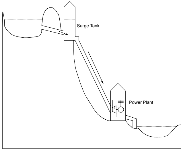
Figure 2.2: Schema of a storage power station
