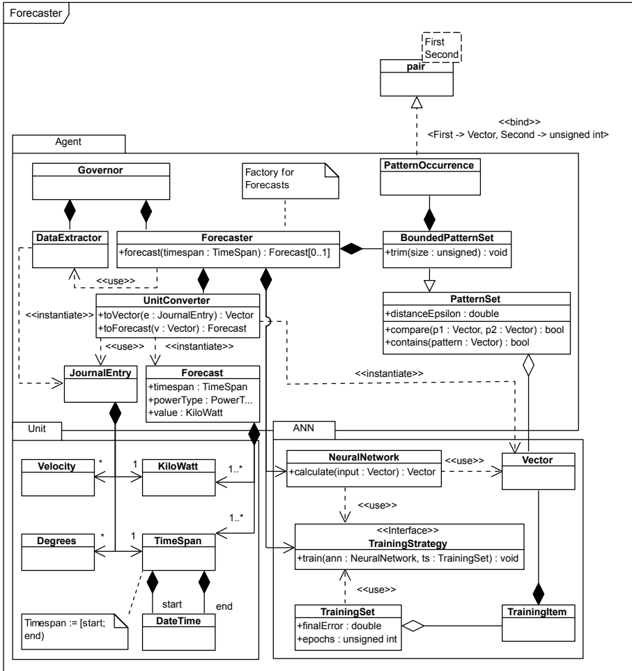
Figure 5.1: Forecaster module of the Universal Smart Grid Agent
