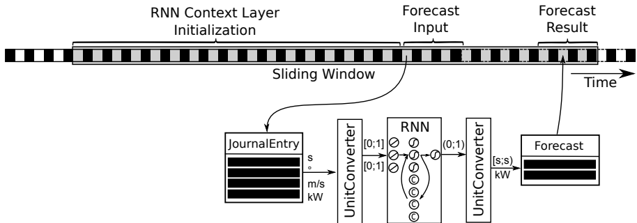
Figure 5.2: The sliding window structure maintained in the forecaster module
