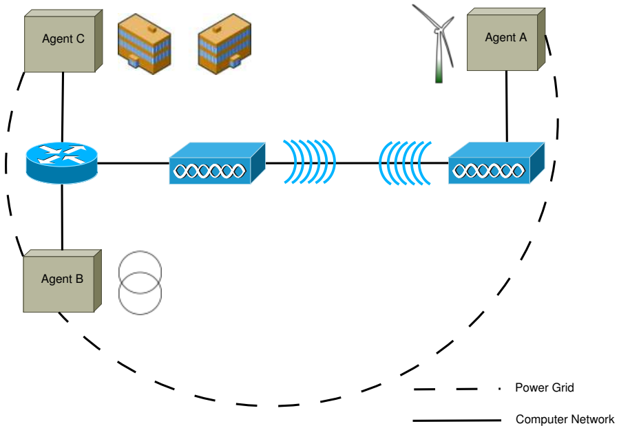
Figure 6.1: The power grid as an overlay network
