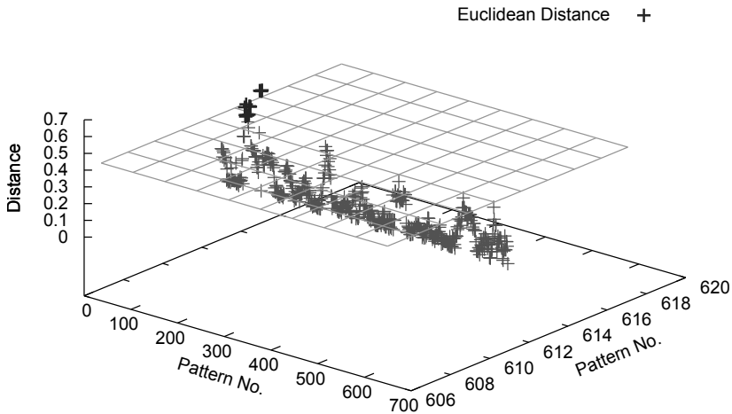
Figure 5.3: Euclidean distances of patterns derived from the reference situation
