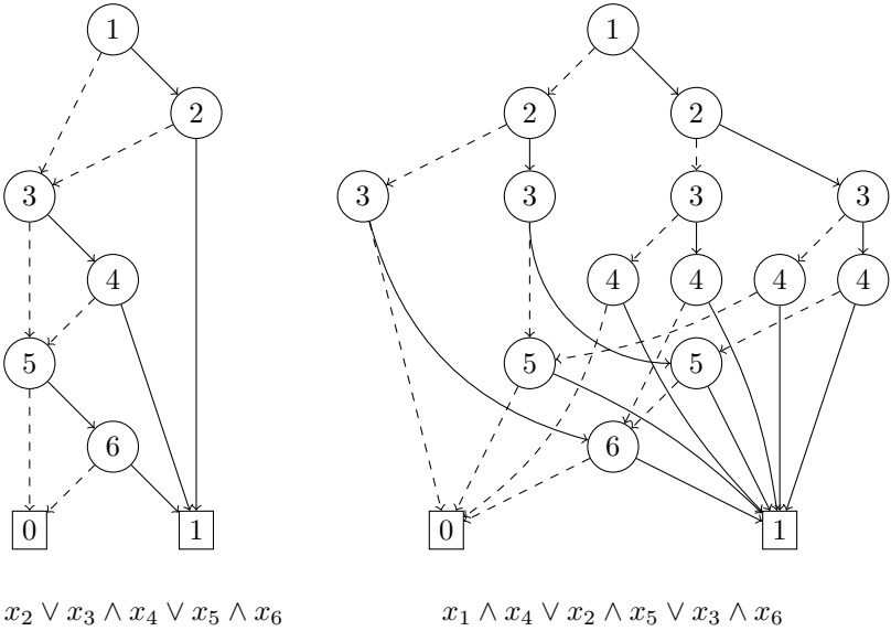
Figure 2.11: Binary Decision Diagrams of two equivalent Boolean functions with different argument ordering
