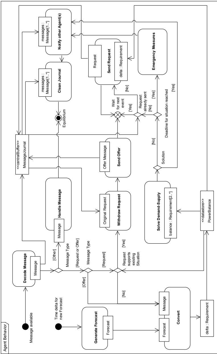
Figure 4.3: Activity diagram depicting the Universal Smart Grid Agent's behavior
