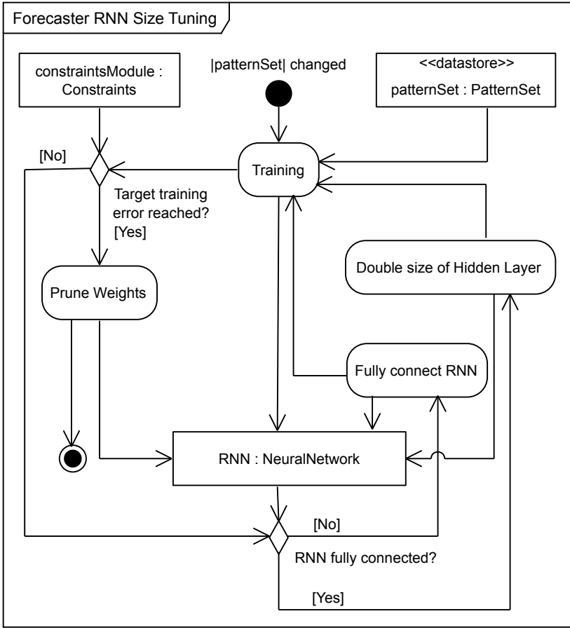
Figure 5.9: Size tuning procedure of the forecaster’s Recurrent Neural Network
