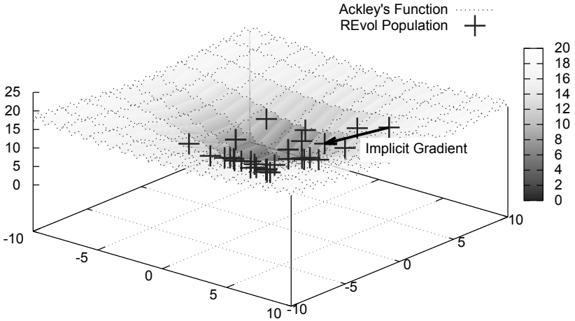
Figure 5.5: Implicit gradient in a REvol population
