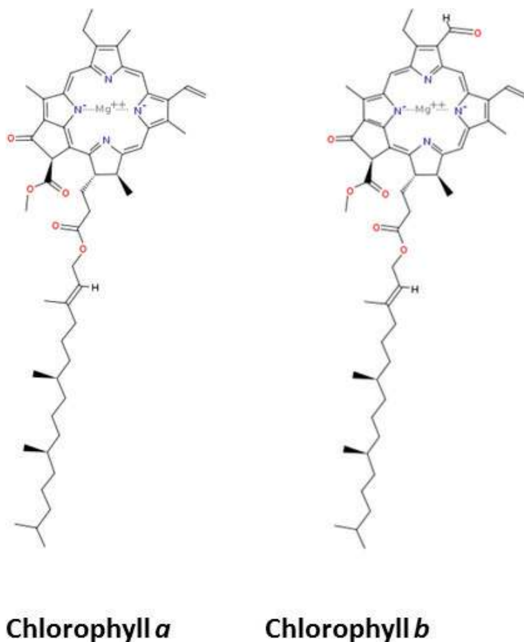
Figure 1. Structures of the chlorophyll molecules.
