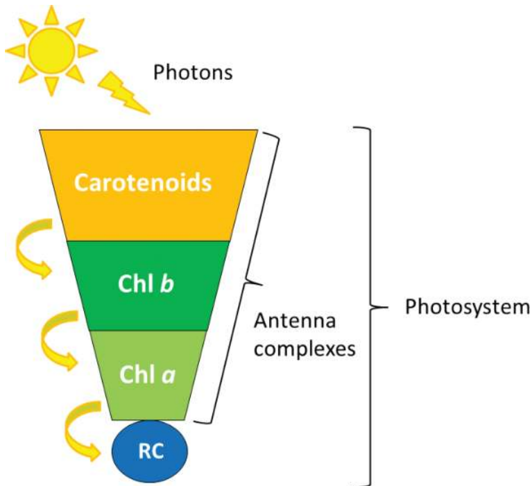
Figure 3. A schematic representation of the light absorption process of chloroplasts. Antenna complexes, composed of carotenoids, Chl a and Chl b molecules, absorb photons from sunlight and transfer them to the RC, which consists of a special couple of molecules of Chl a . Antenna complexes and the RC form a photosystem.
