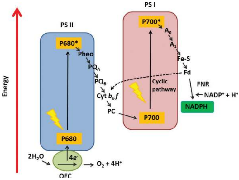
Figure 4. A representation of the linear non-cyclic (solid line) and cyclic electron flow (dashed line) in the chloroplast membranes. OEC tetranuclear Mn cluster; P680, reaction centre of photosystem II (PSII); P680*, excited electronic state of P680; Ph, pheophytin; Q A and Q B , plastoquinone; protein complex containing cytochrome b 6 and cytochrome f; PC, plastocyanin; P700, reaction centre of PSI; P700*, excited electronic state of P700; A 0 , a special chlorophyll a molecule; A 1 , phyloquinone; Fe-S, iron sulphur centres; Fd, ferredoxin; NADP, nicotinamide-adenine dinucleotide phosphate and FNR, ferredoxin-NADP + reductase.
