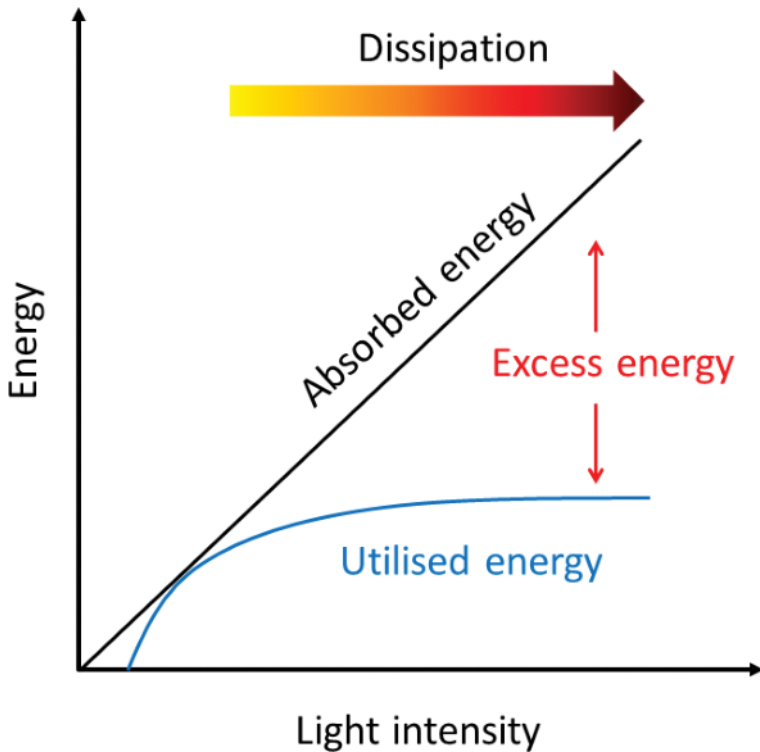
Figure 5. Absorbed and utilized energy in response to increasing light intensities. When light absorbed exceed photo-systems requirement, the 'excess energy' can potentially cause photo-oxidative damage if it is not efficiently dissipated.
