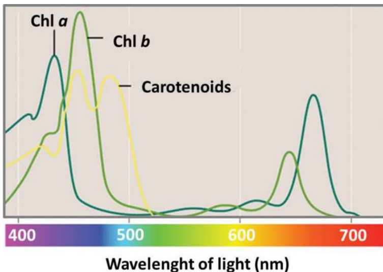
Figure 2. Chlorophyll a , b and carotenoids absorbance spectra.
