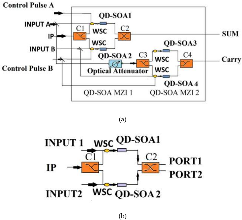
Figure 2. (a). Configuration of the proposed all-optical half-adder using two symmetrical QD-SOA-based MZI switches. (b). XOR gate [25].
