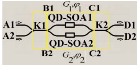
Figure 5. Schematic of SOA-incorporated MZI structure [26].
