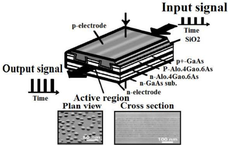
Figure 8. Structure of the quantum-dot SOA with cross-sectional and plan-view images of self-assembled InGaAs quantum dots. [34]
