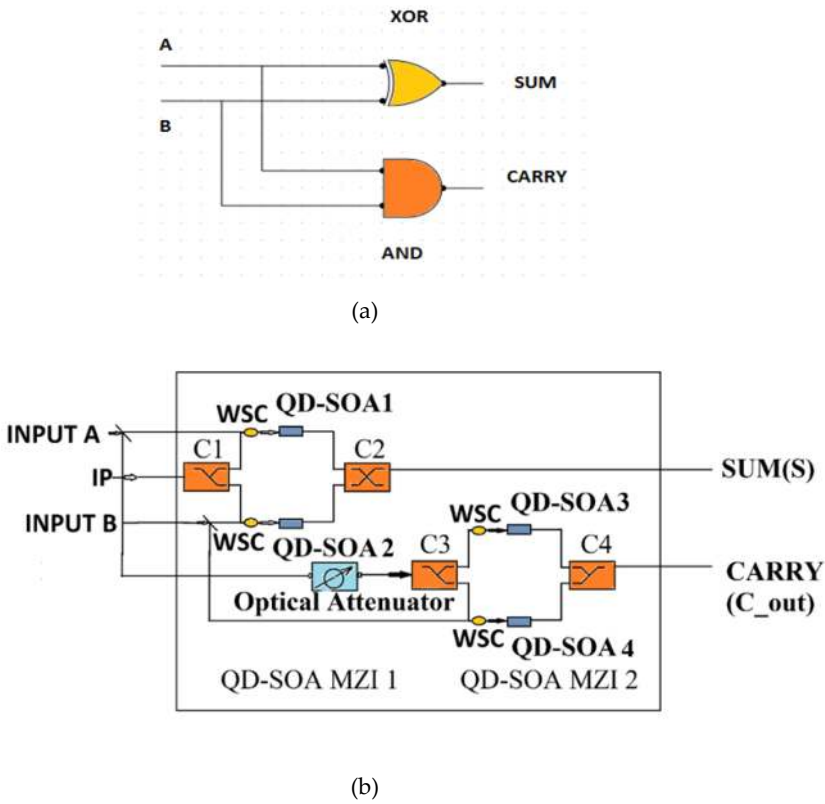
Figure 1. (a). Basic structure of half-adder [14]. (b). Half-adder without control pulse.
