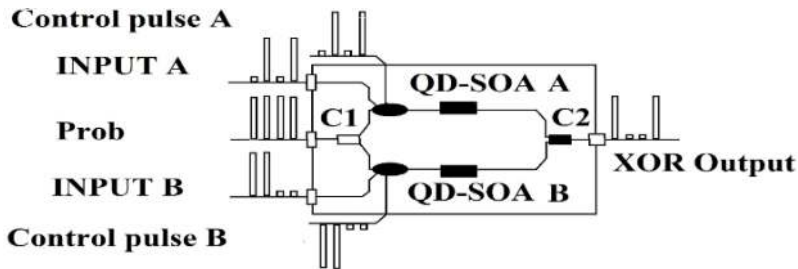
Figure 6. XOR gate based on QD-SOA [3].
