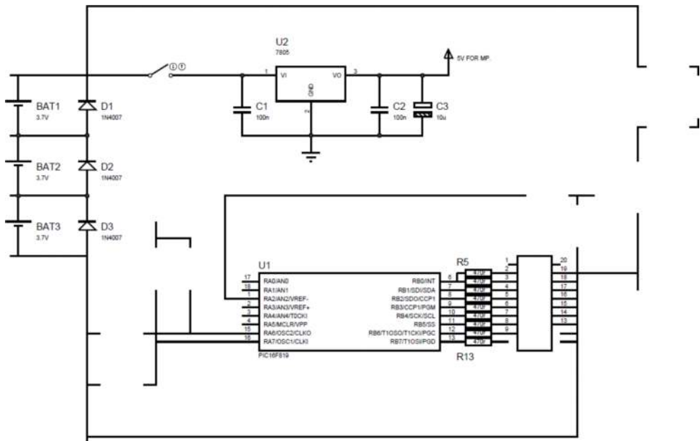
Figure 14. Technical drawing for control module.
