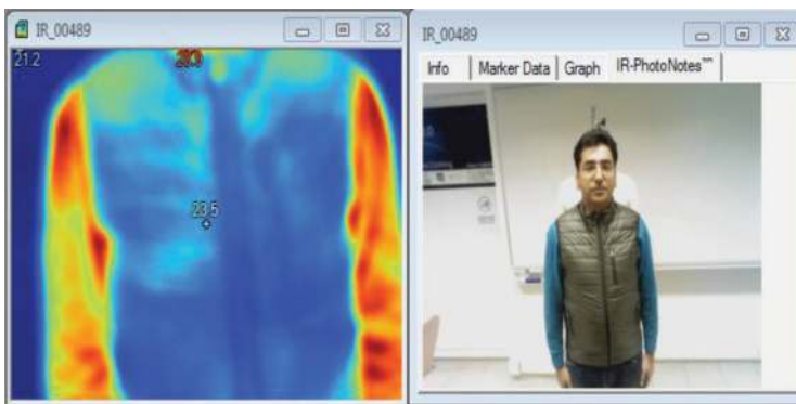
Figure 19. Thermal and actual images on first 30 s after wearing the heating vest (Front surface temperature on the vest: 23.5°C, ambient temperature: 21°C).
