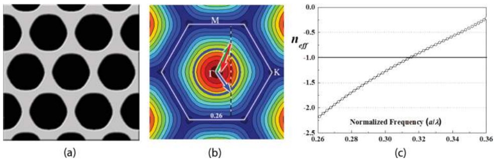
Figure 13. (a) The dielectric pattern of cross section with I_1 = 2.33 ; (b) EFC plot and wave-vector diagram of TM2 band; (c) effective index of TM2 band vs. the normalized frequency.
