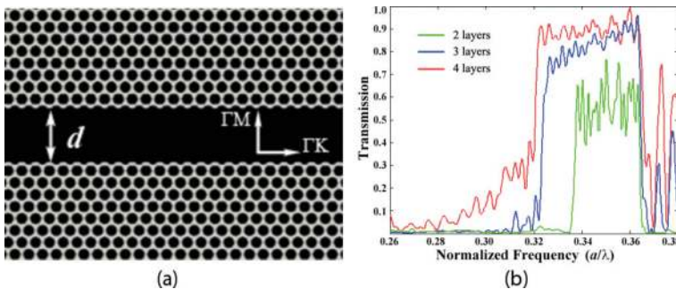
Figure 14. (a) Schematic of the holographic PhC waveguide with a 4 layers width; (b) variation of transmission spectrum for the holographic PCW with different air air width.
