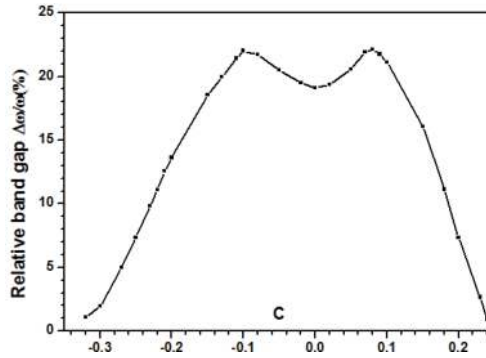
Figure 2. Relation between the value of c and the corresponding maximum relative band width when \epsilon = 13.6 . The two peaks of relative band gap occur at c = -0.1 and 0.08 .
