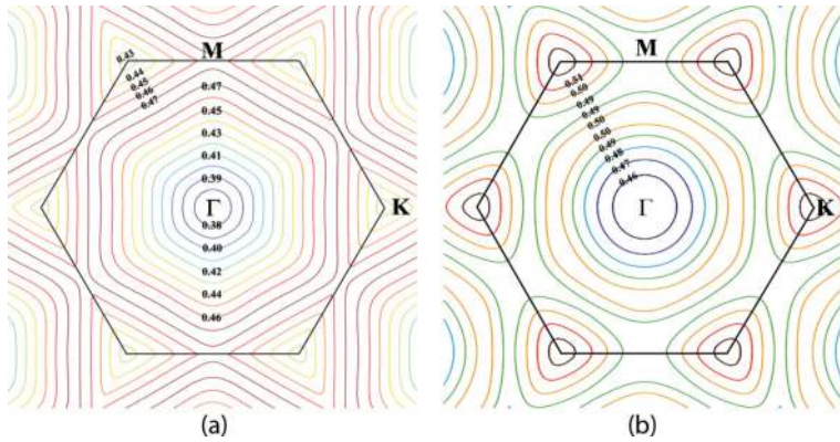
Figure 21. EFC plots of (a) the sixth band and (b) the seventh band.
