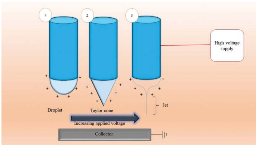
Figure 2. Taylor cone formation stages during voltage application.
