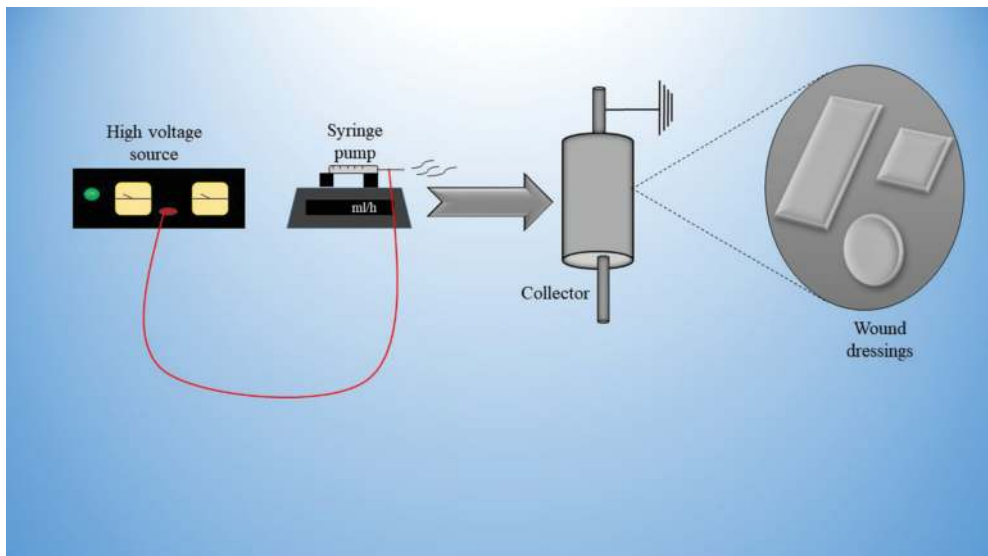
Figure 1. Components of the electrospinning system.
