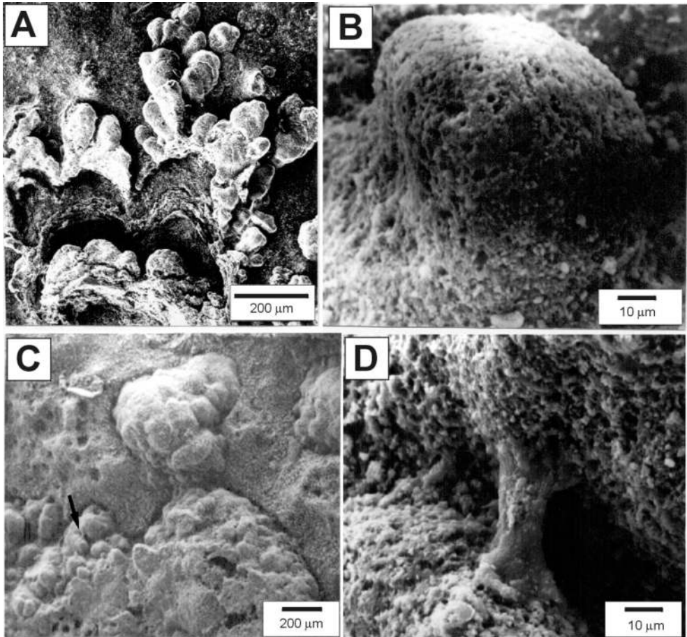
Figure 2. Secondary electron images from phosphate stromatolites. (A) General view of arborescent microstromatolites (etched sample). (B) Cupola formed by francolite. (C) Carbonate-rich sediment located among the phosphate cupolas (arrow points to close-up shown in D). (D) Gelly-like tubular bridge between two phosphate domes; it is made of poorly crystalline P-rich and Si-Al-Fe-rich substances.
