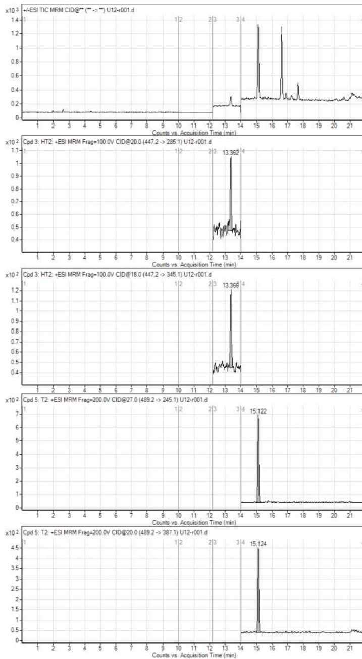
Figure 1. A typical LC-MS/MS-MRM chromatogram of the certified reference material (CRM, oat flour) with values of 77.9 \mu\text{g}/\text{kg} determined for T-2 and 75.6 \mu\text{g}/\text{kg} determined for HT-2; TIC; HT-2 MRM 447.2 \rightarrow 285.1; HT-2 MRM 447.2 \rightarrow 345.1; T-2 MRM 489.2 \rightarrow 245.1; and T-2 MRM 489.2 \rightarrow 387.1.
