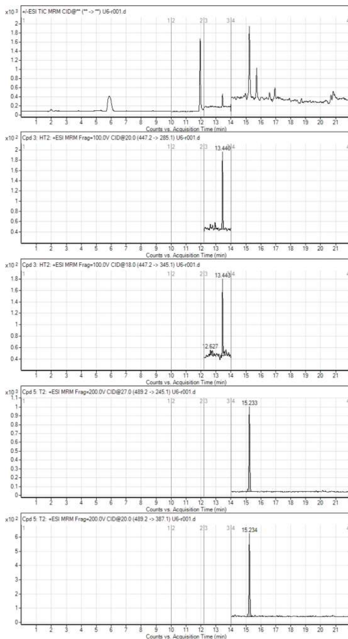
Figure 2. A typical LC-MS/MS-MRM chromatogram of the contaminated maize sample subsequently subjected to thermal reduction processing (128 \mu\text{g}/\text{kg} of T-2 and 256 \mu\text{g}/\text{kg} of HT-2); TIC; HT-2 MRM 447.2 \rightarrow 285.1; HT-2 MRM 447.2 \rightarrow 345.1; T-2 MRM 489.2 \rightarrow 245.1; and T-2 MRM 489.2 \rightarrow 387.1.
