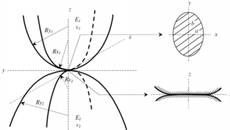
Fig. 4. Geometry of elliptical contact, after Jamari-Schipper (2006)
