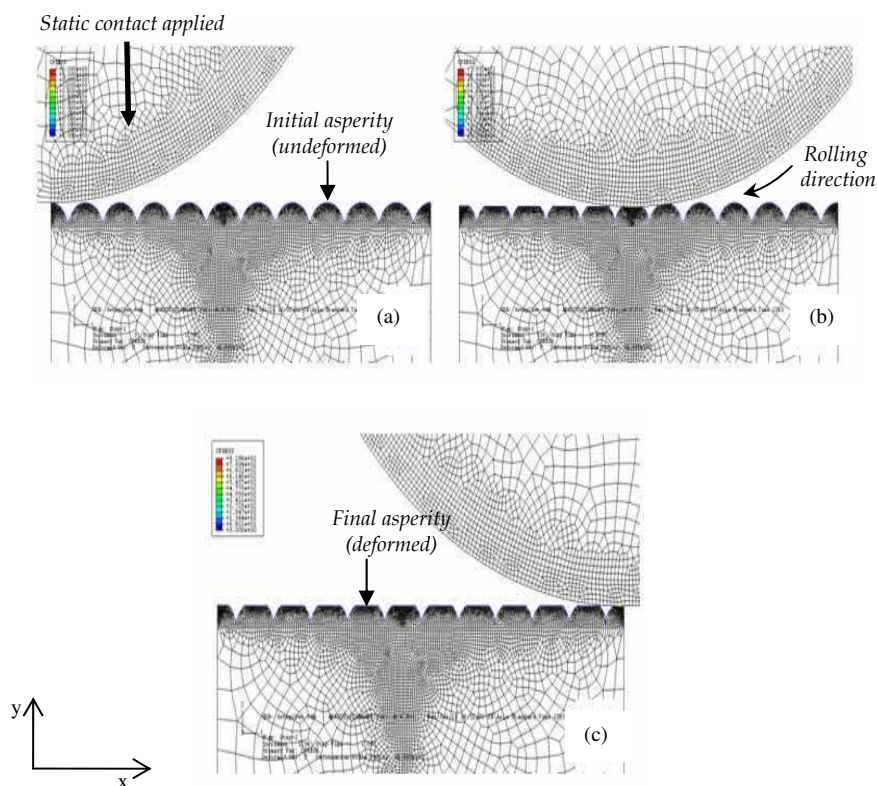
Fig. 6. The rolling contact simulation: (a) start from the static contact, (b) followed by rolling contact with maintaining the contact load, and (c) the roller reaches the end of the rough surface and is unloaded
